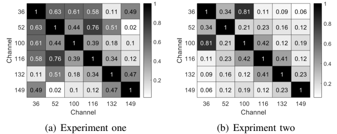
Fig. 17. Channel correlations
