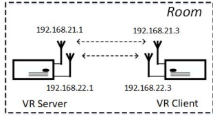
Fig. 2. Networking setup
