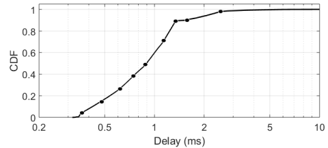
Fig. 10. CDF of channel transmission time
