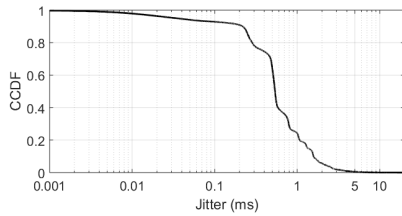
Fig. 5. Complementary CDF of the jitter using single interface
