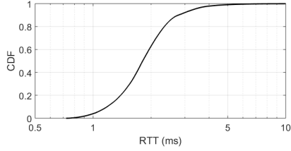
Fig. 4. CDF of the RTT using single interface
