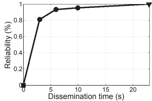
Figure 3: Network reliability of Splash at some specific time points. The end of 3 dissemination rounds is indicated by circle markers. The local recovery phase is from the end of the third round till the last node correctly receives the data object.
