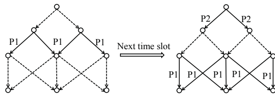
Figure 1: The pipelined tree built on constructive interference and pipelining. ‘P1’ and ‘P2’ represent the first packet and the second packet respectively.
