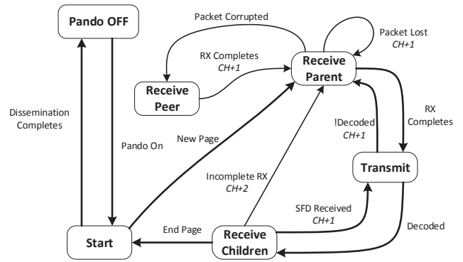
Figure 7: Node state machine in Pando.
