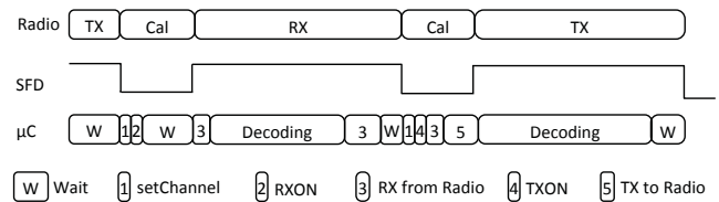
Figure 4: State transition of the radio and the microcontroller in Pando.
