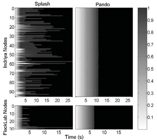
Figure 8: Reliability of individual nodes achieved by Pando and Splash on Indriya and Flocklab.
