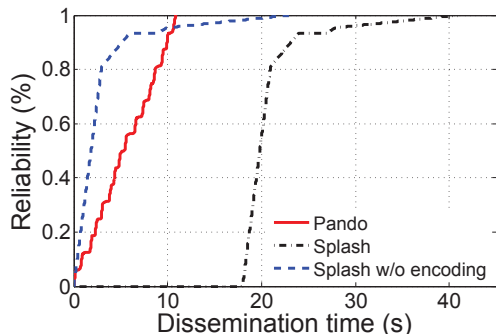
Figure 9: Network reliability progress on Indriya.
