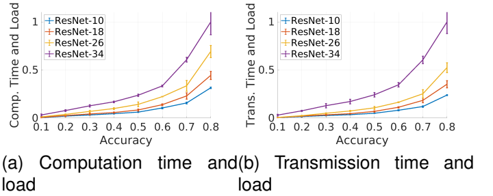
Fig. 5. CompT, TransT, CompL, and TransL versus model complexity. The lower the better.
