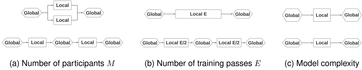
Fig. 6. Intuitive explanation of our measurement results. (a) The number of participants. The bottom scheme is better regarding CompL and TransL. (b) The number of training passes. The bottom scheme is better regarding CompT and CompL. (c) Model complexity. The bottom scheme is better for CompT, CompL, TransT, and TransL.
