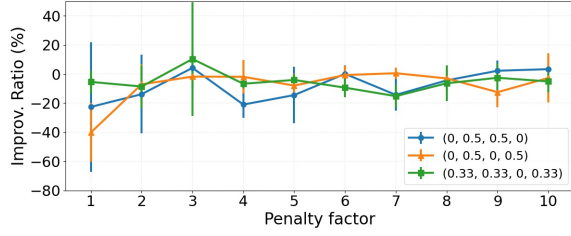
Fig. 8. Performance of the degraded cases versus the penalty factor. Speech-to-command dataset and FedAvg is used in this experiment. In particular, FedTune reduces the system overhead of FedAdagrad by 26.75%.
