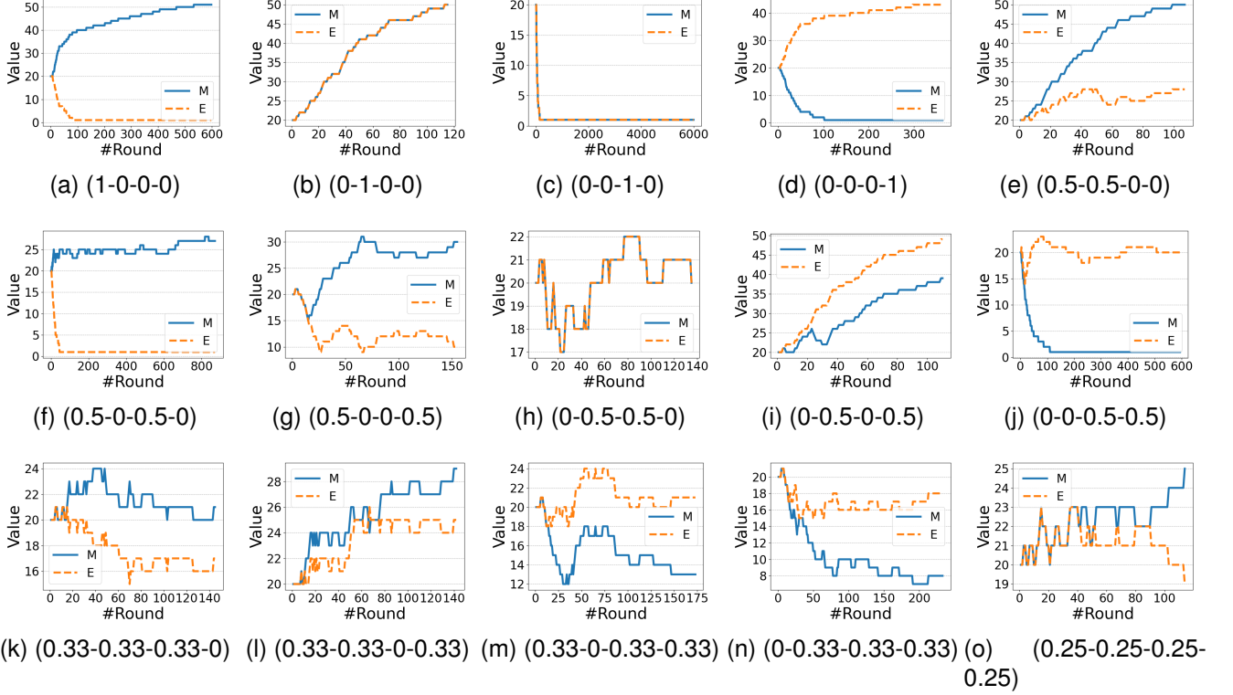
Fig. 7. Illustrations of the number of participant M and the number of training passes E during FL training for different application preferences.
