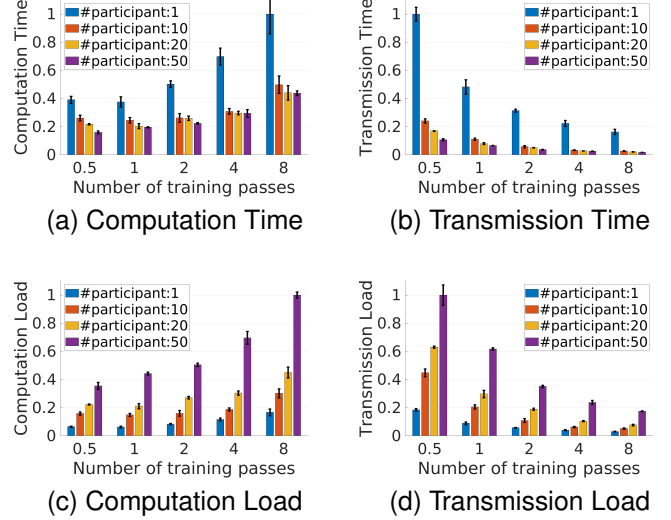
Fig. 4. CompT, TransT, CompL, and TransL when a different number of participants and a different number of training passes are used. The lower the better.
